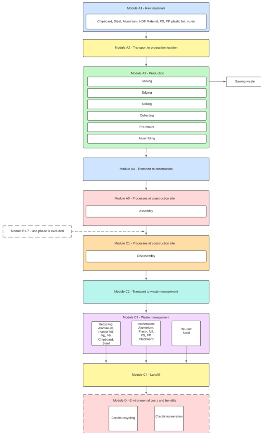
LCA process diagram according to EN 15804 (7.2.1)
